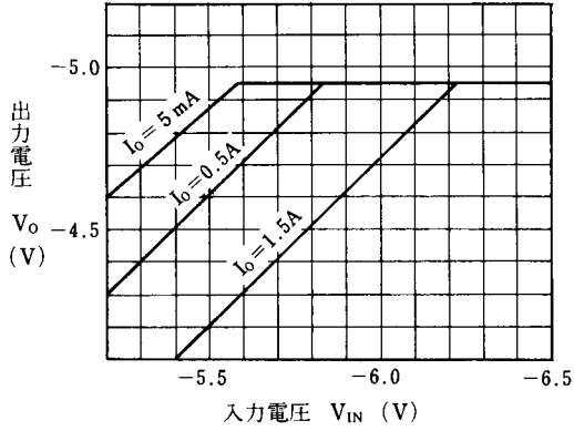
NJM7905 入出力間電位差特性例 ( T_j = 25^\circ\text{C} )
