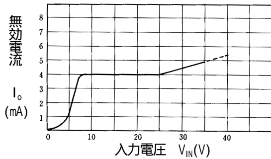
NJM78M05 無効電流特性例 ( I_o = 0\text{mA} , T_j = 25^\circ\text{C} )
