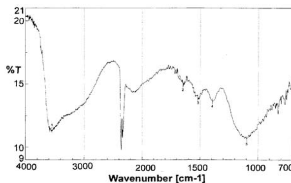
Fig.2. FT-IR analysis on the floating materials shown in Fig.1 indicates absence of chemical bond of C-H. But there exists bond of \text{H}_2\text{O} and that of \text{CO}_2 .
