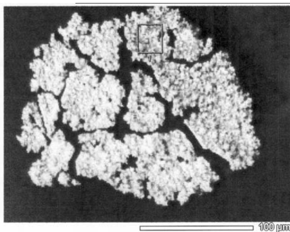
Fig.3 The mapping for EDS analysis by SEM(x500). A small square indicated in Fig.3 is region (1).
