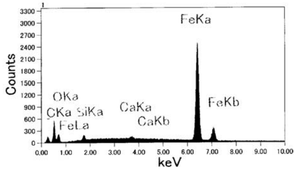
Fig. 4. EDS X-ray spectrum for region (1).
