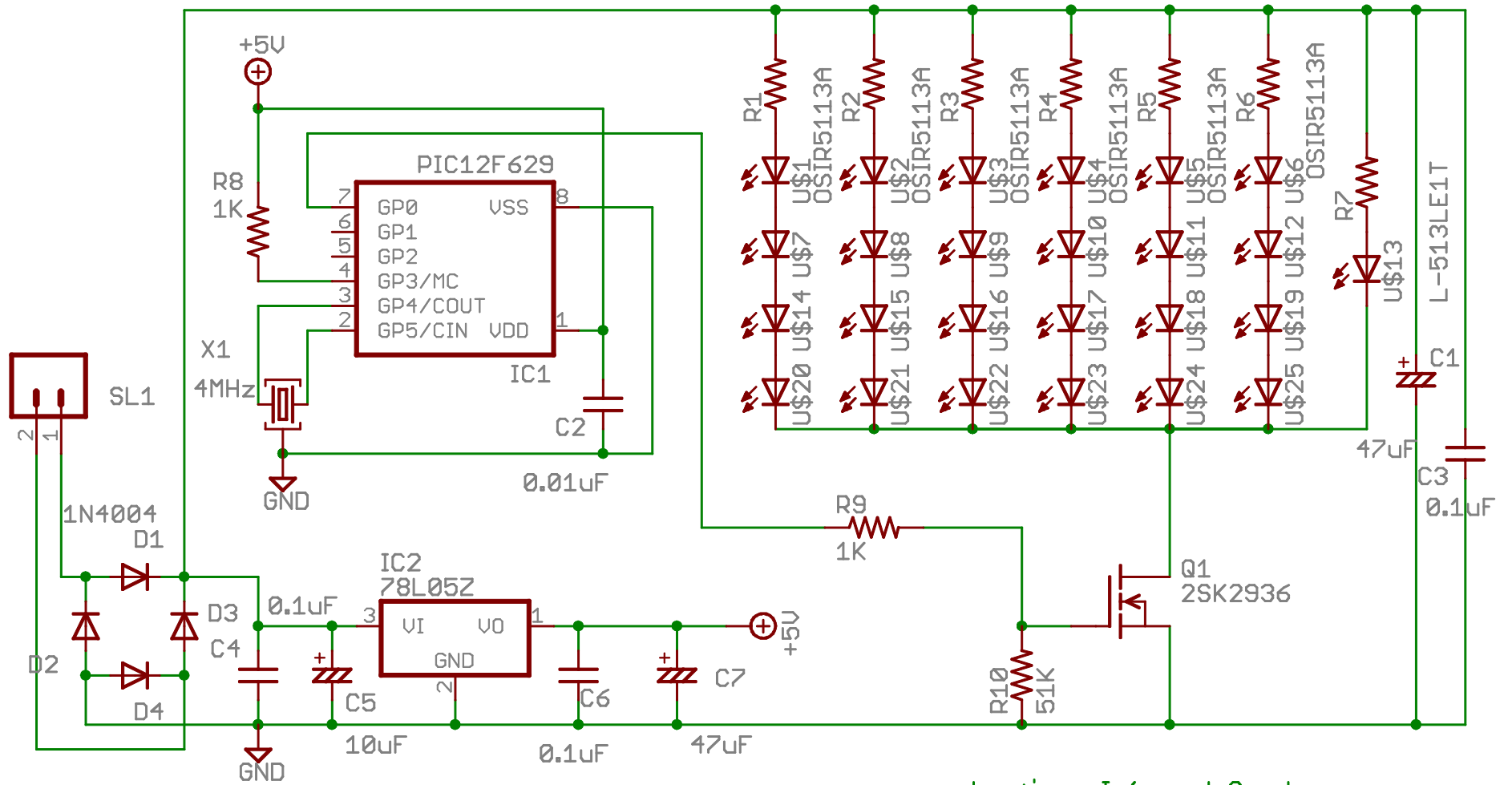
Laptimer Infrared Sender July 16, 2005 (c) Kenji Arai /JH1PJL
