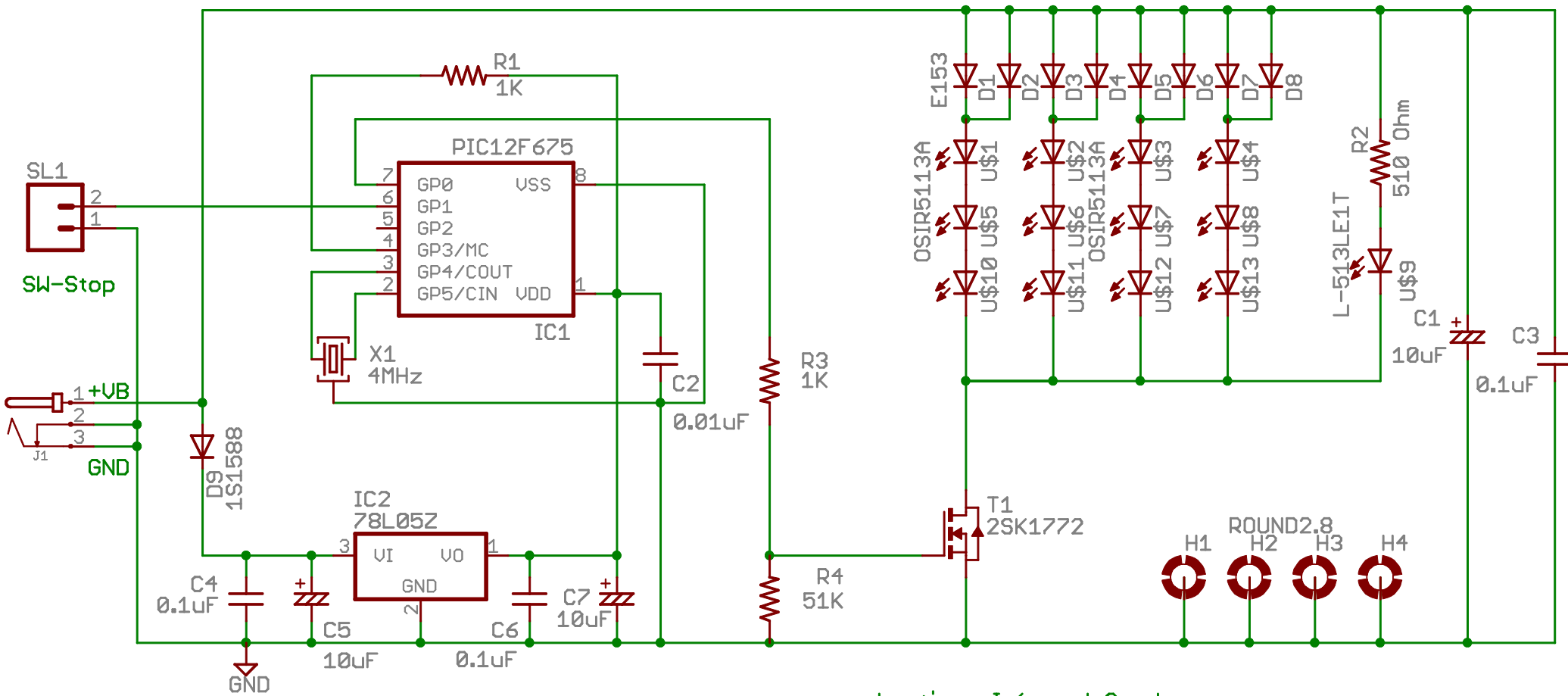
Laptimer Infrared Sender Gymkhana Version (c) Kenji Arai /JH1PJL January 4th, 2007
