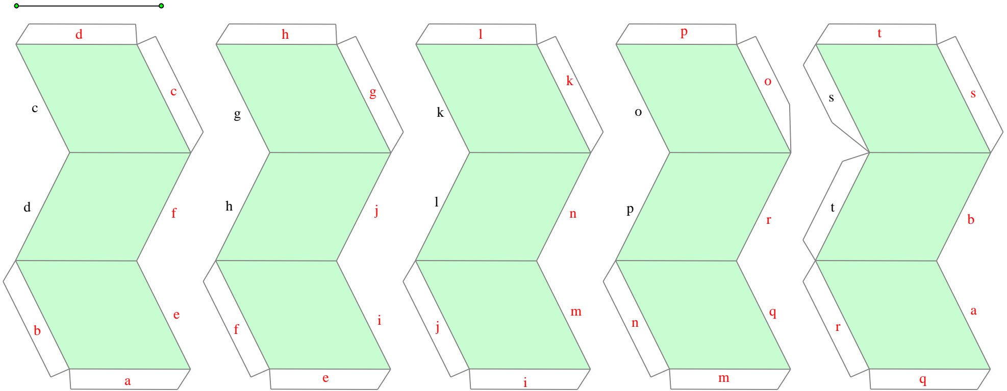
[3,5,3,5] Rhombic-triacontahedron 菱形三十面体 (2枚目)
