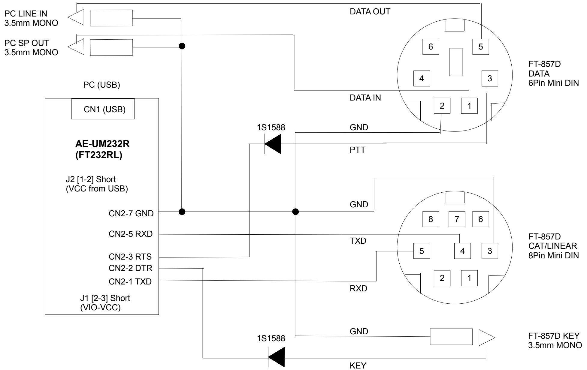
FT-857 USB RIG CONTROL, ELEKEY, and RTTY I/F
